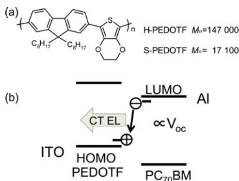
Figure 1. (a) Chemical structure of PEDOTF. H-PEDOTF with M_n of 147,000 prepared via direct C-H arylation and S-PEDOTF with M_n of 17,100 prepared via the Suzuki-Miyaura cross-coupling reaction. (b) Conceptual energy diagram of this study.
