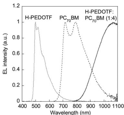
Figure 2. EL spectra from OLEDs with H-PEDOTF, PC 70 BM, and the H-PEDOTF:PC 70 BM (1:4) blended (BHJ) layer.
