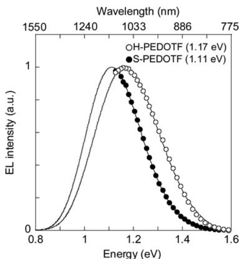
Figure 3. CT ET spectra from the BHJ layers of H-PEDOTF:PC 70 BM and S-PEDOTF:PC 70 BM (1:4). The values shown in parentheses are the energies of CT EL peaks. The solid lines are Gaussian fitted curves of obtained CT EL spectra.
